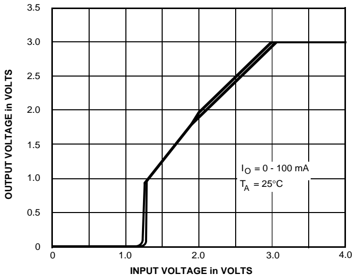
OUTPUT VOLTAGE
