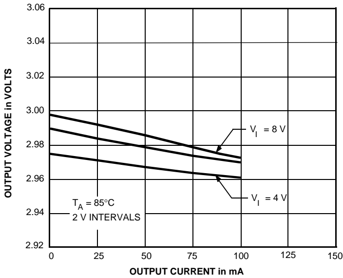
LOAD REGULATION
