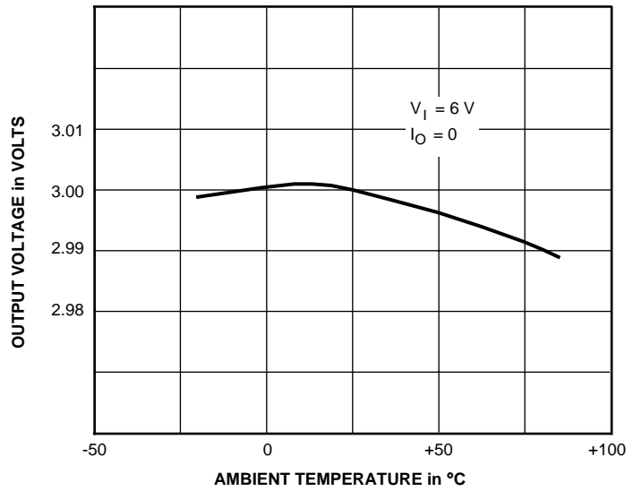
OUTPUT VOLTAGE
