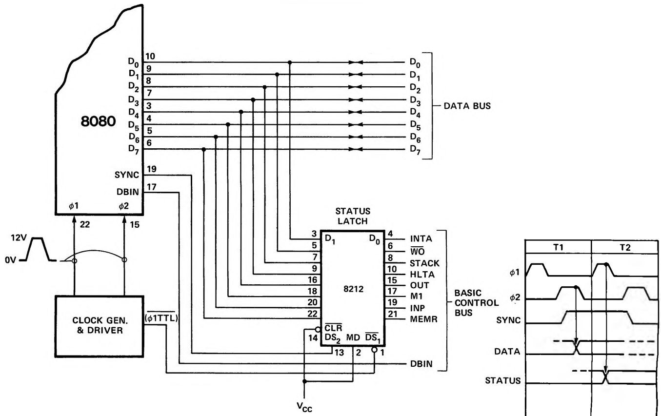
8080 STATUS LATCH
