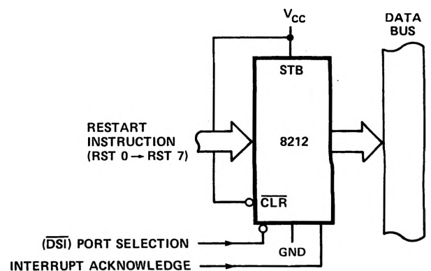
INTERRUPT INSTRUCTION PORT
