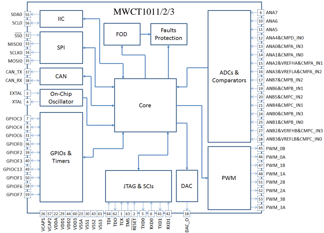
Figure 1. WCT1011/3VLH and WCT1012VLF function block diagram
