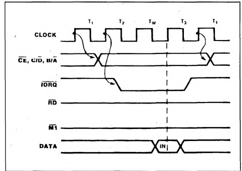
Figure 18 : Write Cycle.
