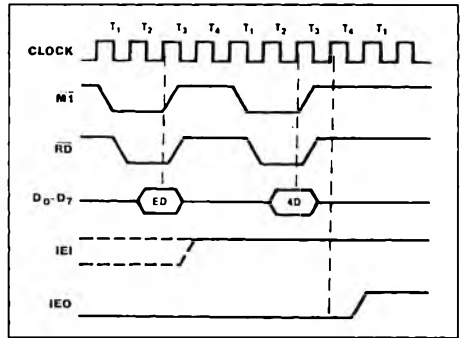
Figure 20 : Return from Interrupt Cycle.
