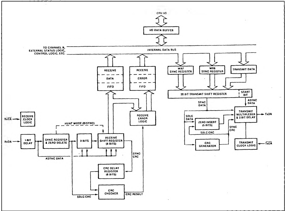
Figure 14 : Transmitt and Receive Data Path (channel A).
