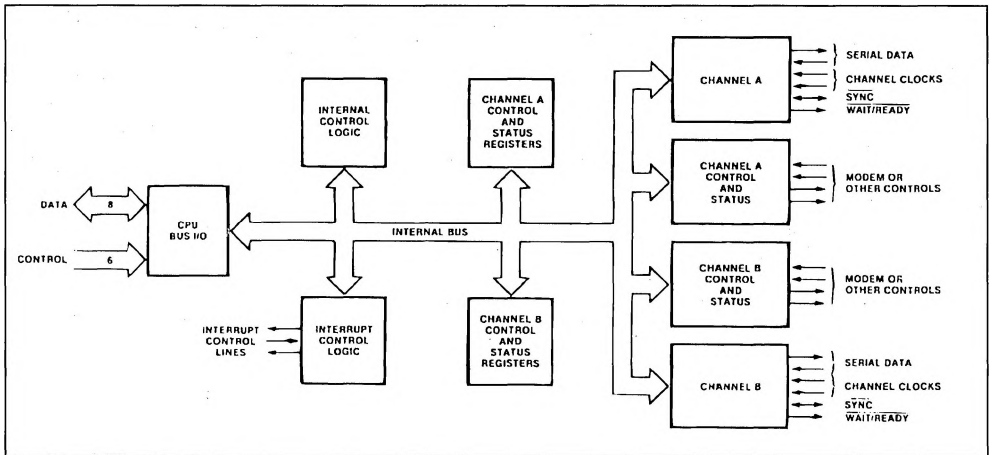
Figure 8 : Block Diagram.
