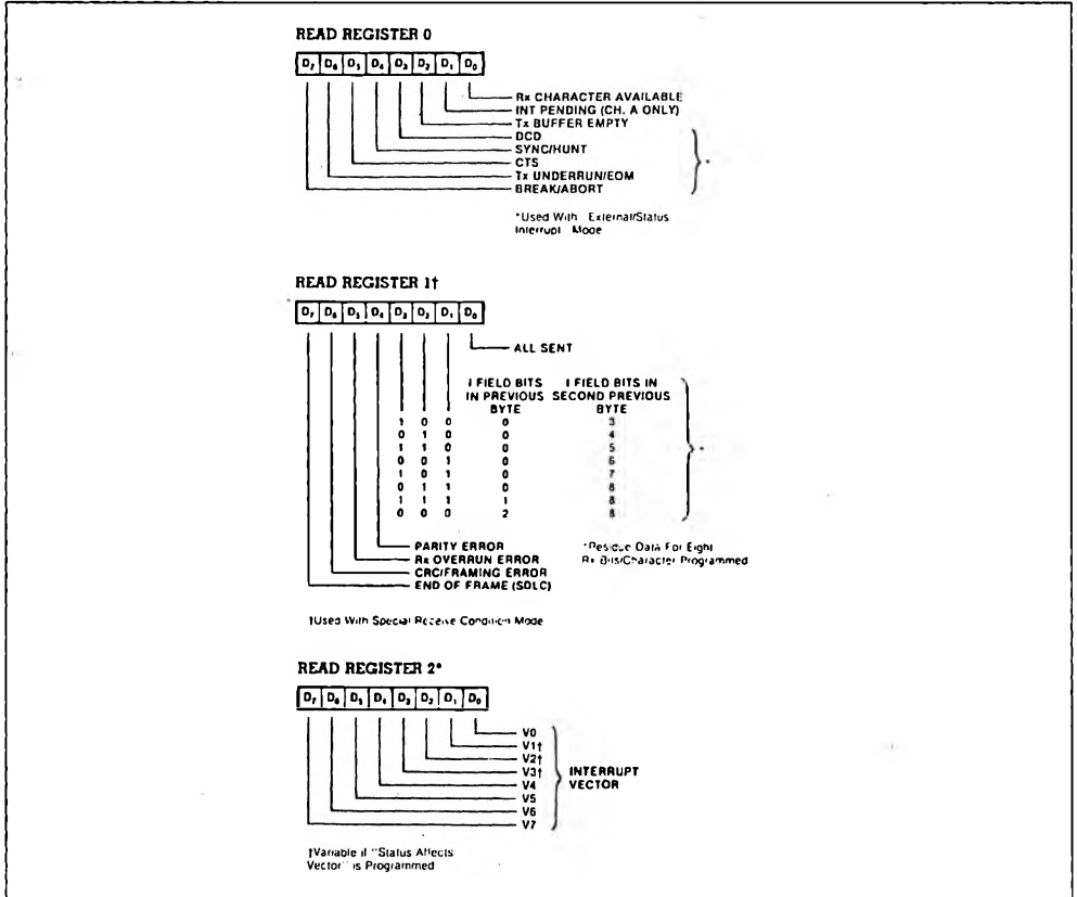
Figure 15 : Read Register Bit Functions.
