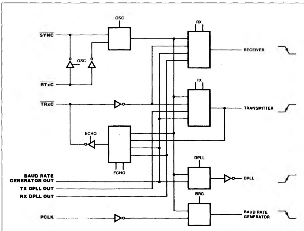
Figure 32 : Clock Multiplexer.
