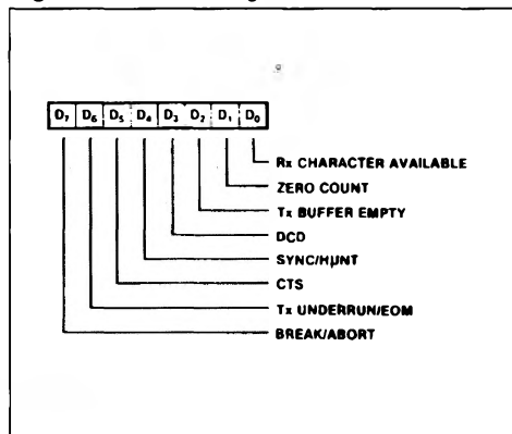
Figure 59 : Read Register 0.
