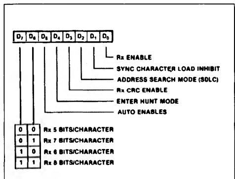
Figure 46 : Write Register 3.
