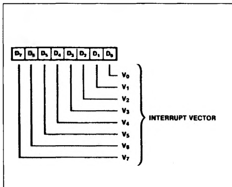
Figure 61 : Write Register 2.
