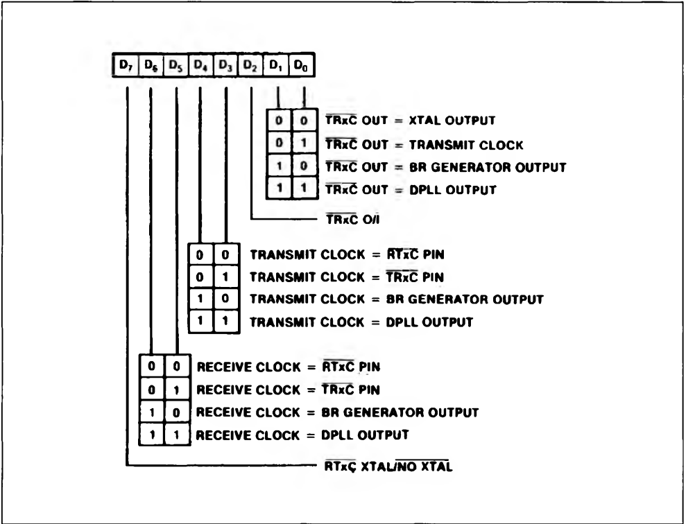
Figure 54 : Write Register 11.
