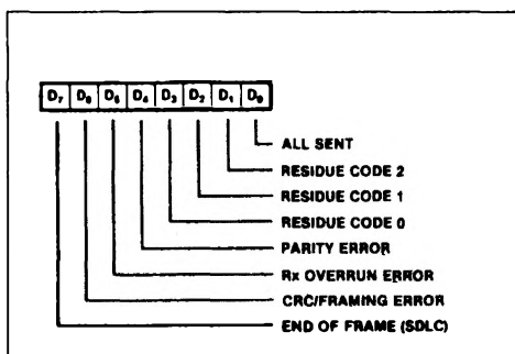
Figure 60 : Read Register 1.
