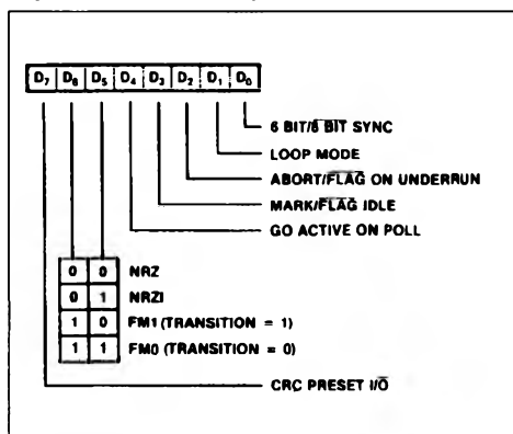
Figure 52 : Write Register 10.
