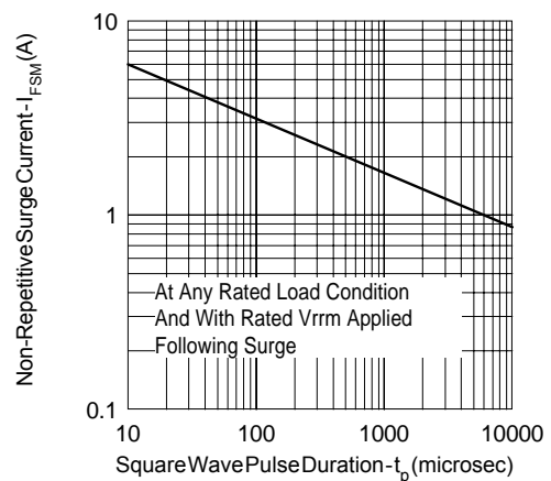
Fig. 5 - Max. Non-Repitative Surge Current
