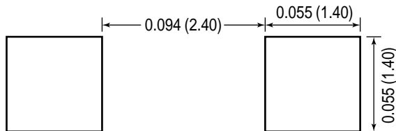
Mounting Pad Layout SOD-123 (BB721)
