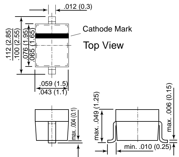
SOD-323 (BB721S)
