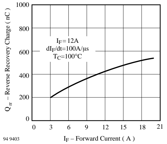
Figure 7. Reverse Recovery Charge vs. Forward Current
