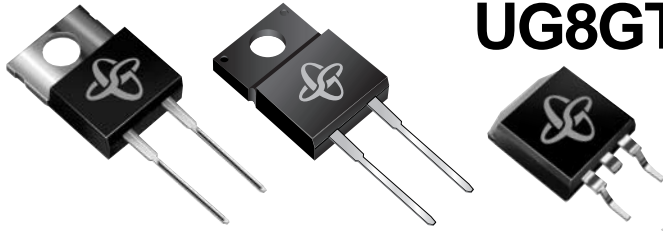
TO-220AC (BYV29, UG8 Series)
