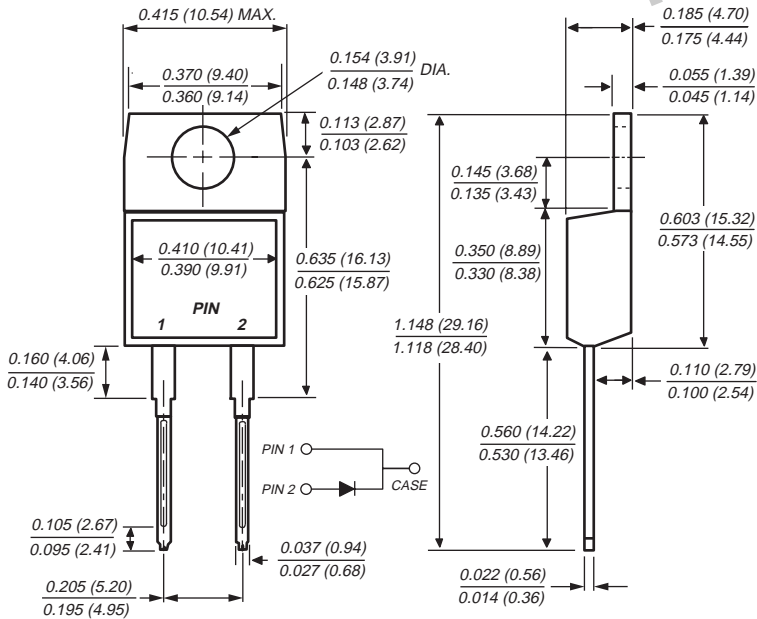
TO-220AC (BYV29, UG8 Series)
