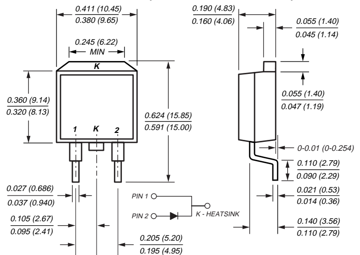
TO-263AB (BYV29B, UGB8 Series)
