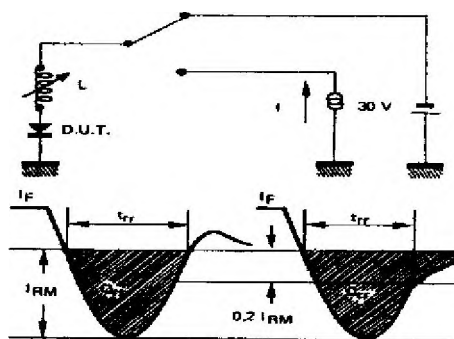
Figure 10. Measurement of t_{rr} (Fig. 7) and I_{RM} (Fig. 8).
