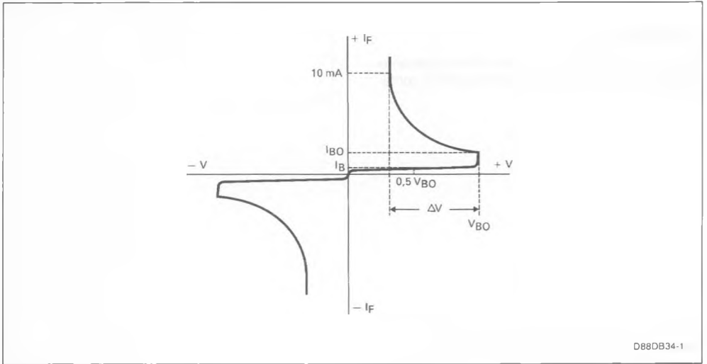
DIAGRAM 1 : Current-voltage characteristics.
