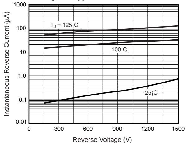
Fig. 4 – Typical Reverse Current
