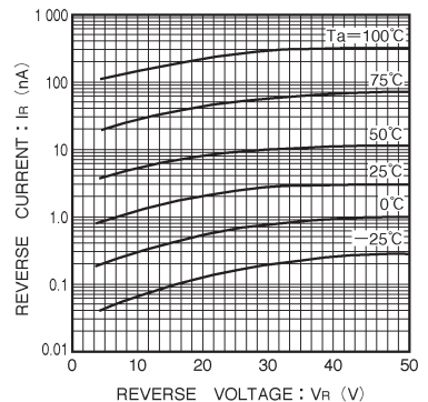
Fig. 3 Reverse current vs. reverse voltage (P TYPE)
