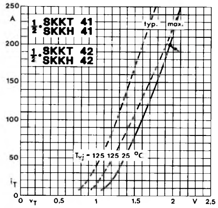
Fig. 8 On-state characteristics
