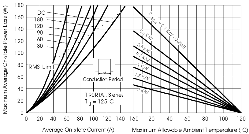
Fig. 29 - On-state Power Loss Characteristics
