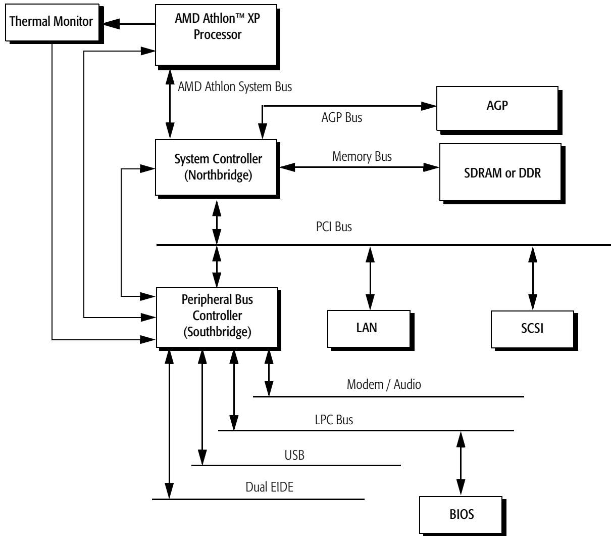
Figure 1. Typical AMD Athlon™ XP Processor System Block Diagram
