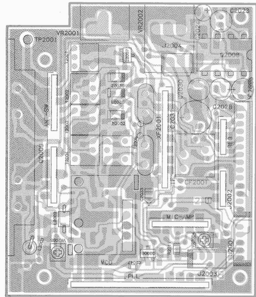
obverse view "component" side
