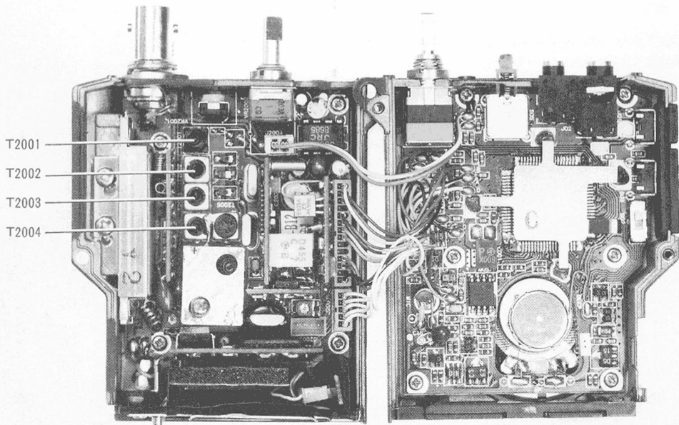
RECEIVER SECTION ALIGNMENT POINTS
