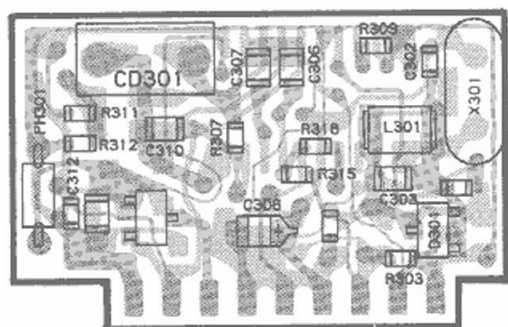
obverse view "mixed-component" side
