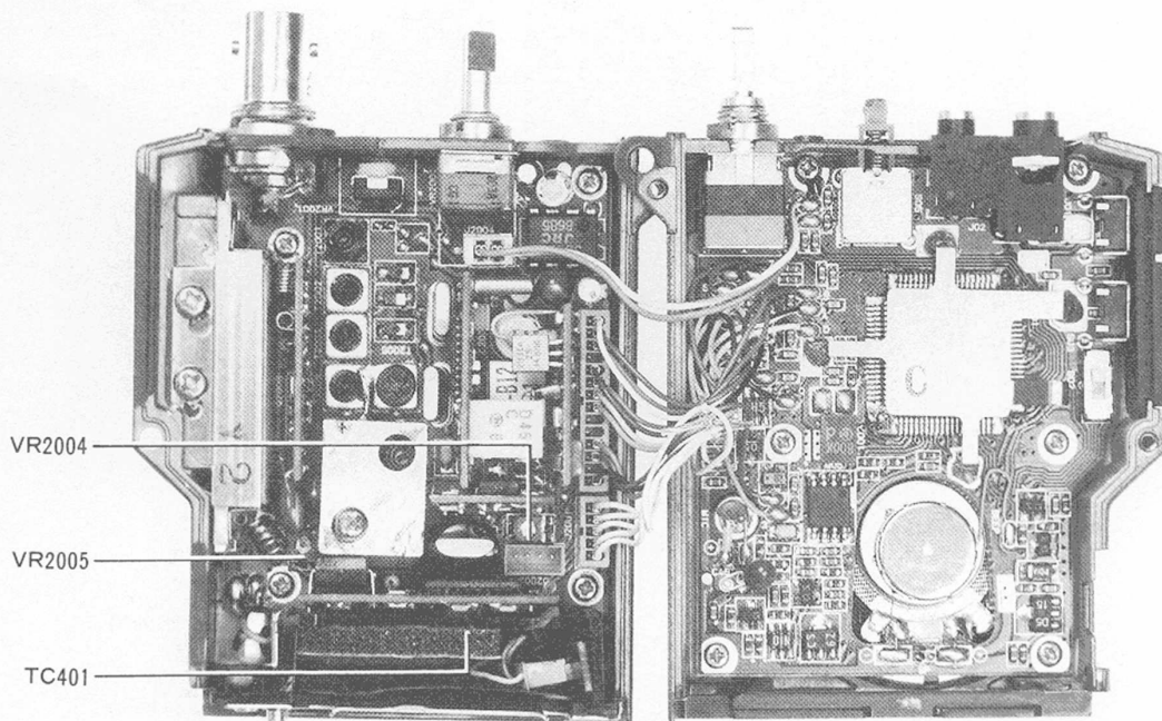
TRANSMITTER SECTION ALIGNMENT POINTS
