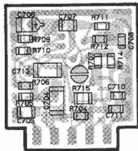
obverse view "chip-only" side
