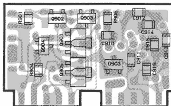
obverse view "chip-only" side
