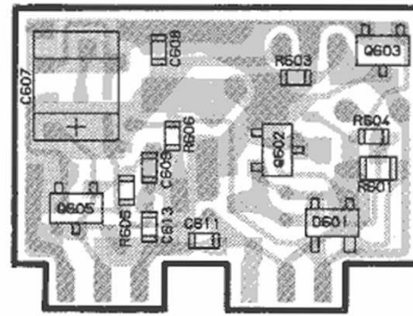
obverse view "chip-only" side
