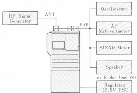
RECEIVER ALIGNMENT SETUP
