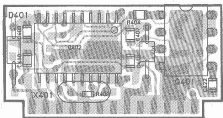
obverse view "mixed-component" side
