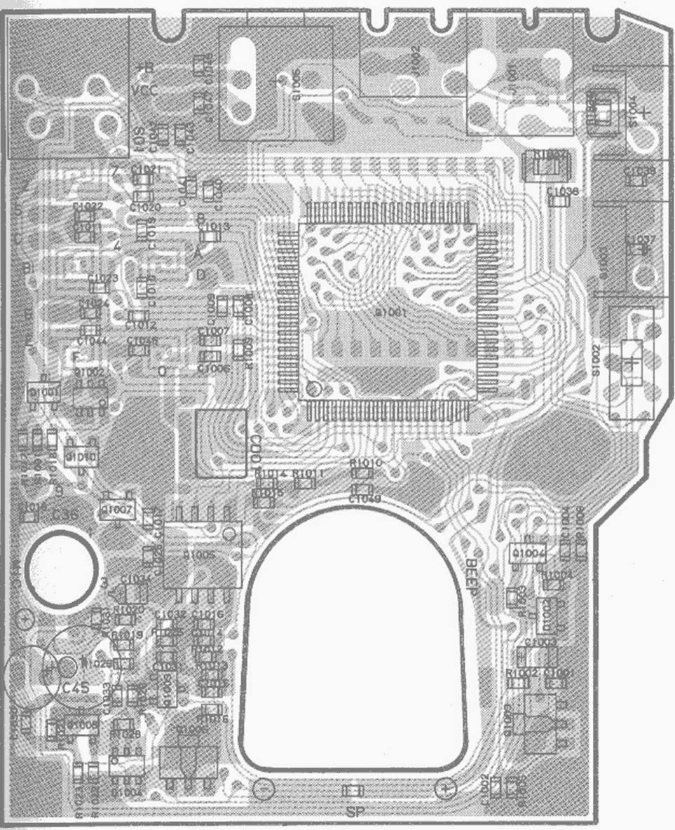
obverse view "mixed-component" side
