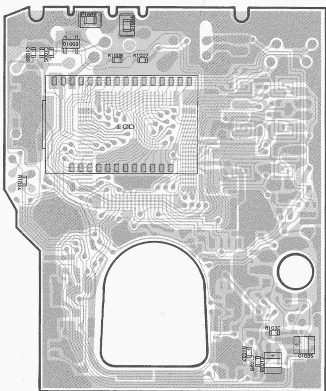
obverse view "chip-only" side
