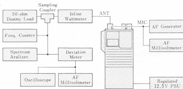
TRANSMITTER ALIGNMENT SETUP
