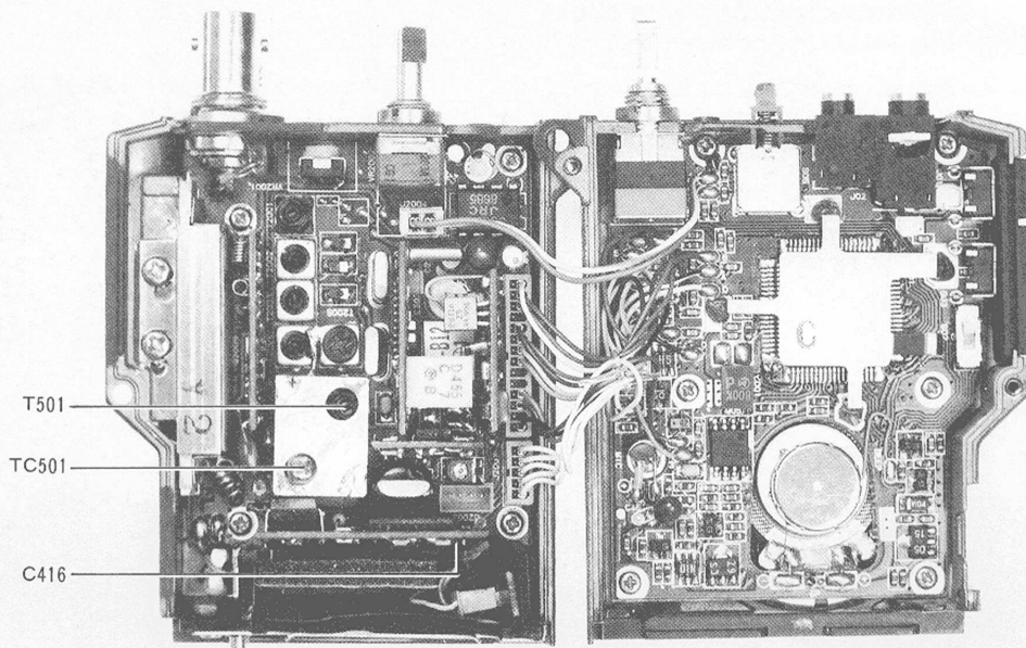
PLL SECTION ALIGNMENT POINTS
