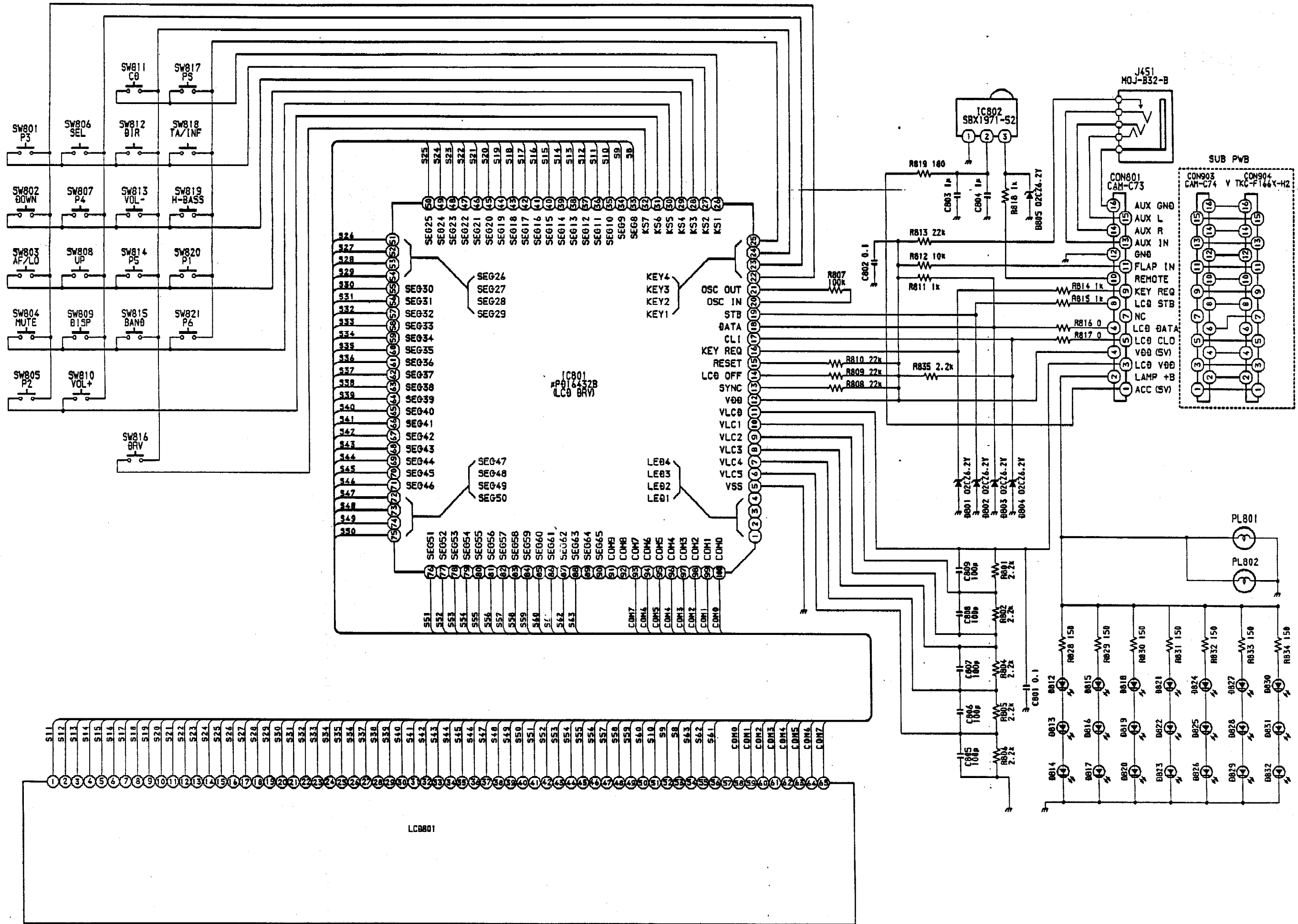
SCHEMATIC DIAGRAM - 2 (FRONT)
